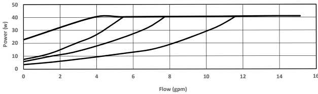
PROPORTIONAL PRESSURE
