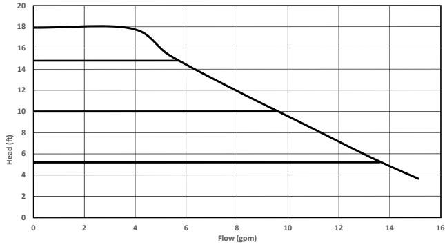
CONSTANT SPEED
