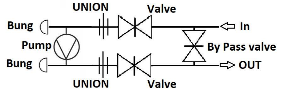
Option 2 pipe in and out on the right
