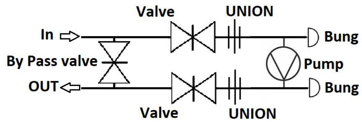
Option 1 pipe in and out on the left
