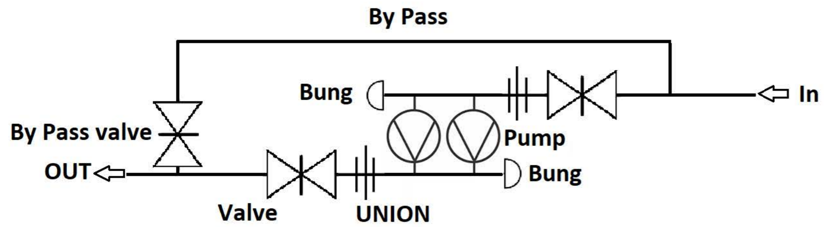
Option 3 pipe in on the right and out on the left
