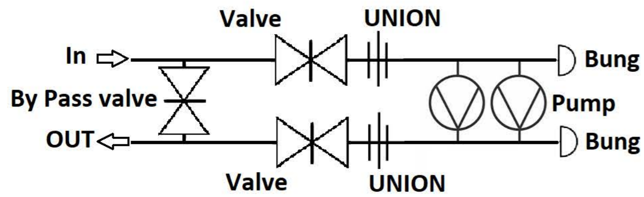
Option 1 pipe in and out on the left
