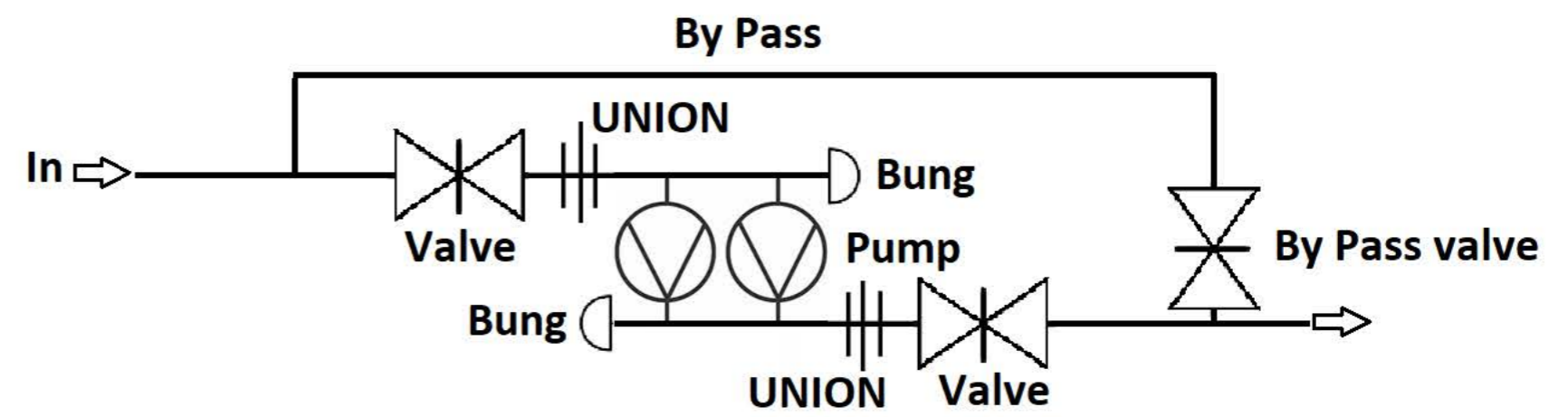
Option 4 pipe in on the left and out on the right
