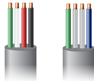
POWER CABLE SENSOR CABLE
